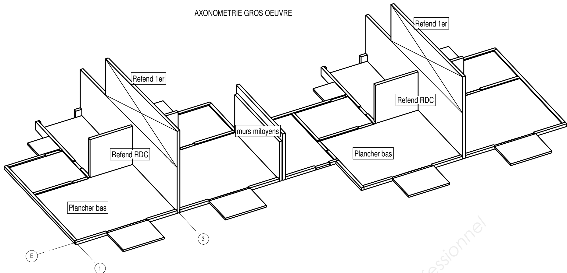
PLAN SOLIVAGE R+1 Echelle 1/50
